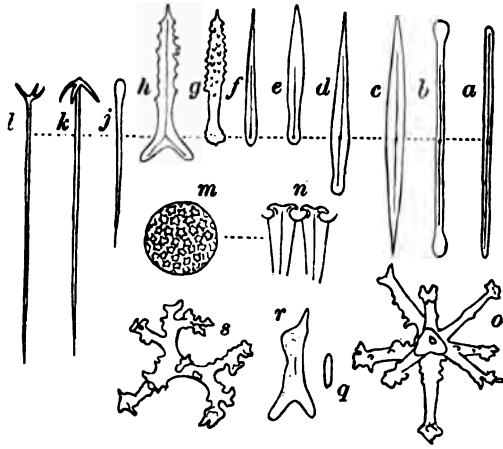
FIG. 110.—Megascleres. a-l and q-s , Modifications of monaxon type. a , Strongyle; b , tylote; c , oxea; d , tylotoxea; e , tylostyle; f , style; g , spined tylostyle; h , sagittal triod (a triaxon form derived from monaxon); j , oxytylote; k , anatriaene; l , protriaene; m , sterraster (polyaxon); n , radial section through the outer part of m , showing two actines soldered together by intervening silica; o , desma of an Anomocladine Lithistid (polyaxon); q , crepidial strongyle, basis of rhabdocrepid Lithistid desma; r , young form of rhabdocrepid desma, showing crepidial strongyle coated with successive layers of silica; s , rhabdocrepid desma.
